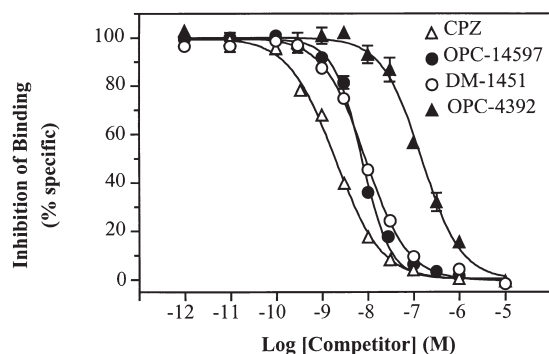
Figure 2. Affinity of OPC-14597 and selected reference compounds for dopamine D_2 -like receptors in rat striatal membranes. Dopamine D_2 receptors were labeled with 0.07 nM [ ^3H ]-spiperone in the presence of 50 nM ketanserin to mask 5-HT _2 sites. Nonspecific binding was defined by 1 \mu M chlorpromazine (CPZ). For each compound, at least three independent assays were conducted on separate days. The curves shown are from representative experiments. Means and standard errors are shown in Table 1.
