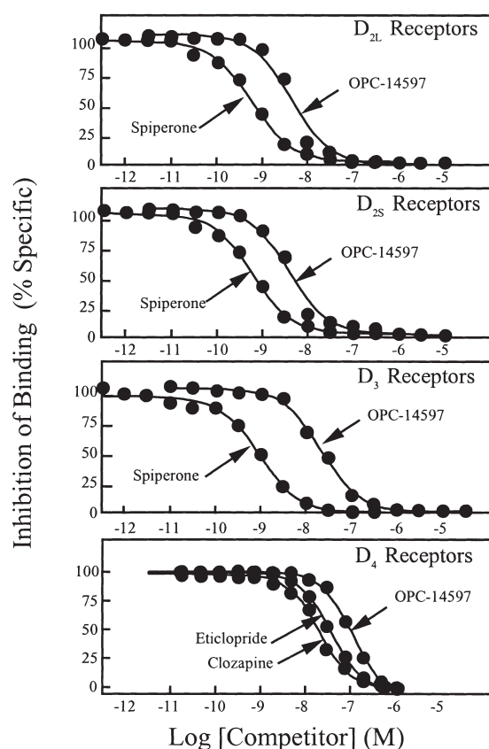
Figure 3. Affinity of OPC-14597 for cloned D_2 -like dopamine receptors in CHO cells. Membranes were prepared from CHO cells stably transfected with dopamine D_{2L} , D_{2S} , D_3 , or D_4 receptors. Receptors were labeled with 0.2 nM [ ^3H ]-methylspiperone. Nonspecific binding was defined by 1 \mu M (+)-butaclamol. For each compound, at least three independent assays were conducted on separate days. The curves shown are from a single representative experiment. Means and standard errors for receptor affinities ( K_{0.5} ) are shown in Table 2.
